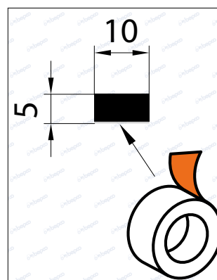
MOUSSE ADHESIVE EP5X10
