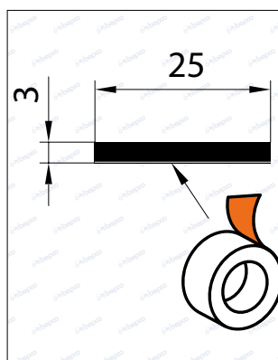
MOUSSE ADHESIVE EP3X25
