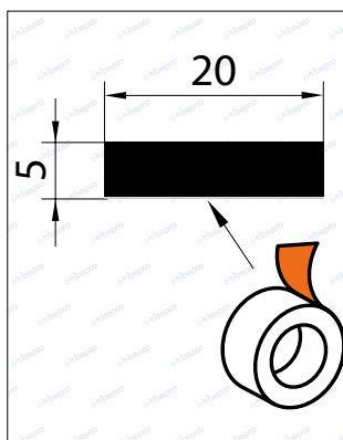
MOUSSE ADHESIVE EP5X20
